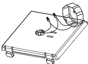
Fig.A(J-Box)
